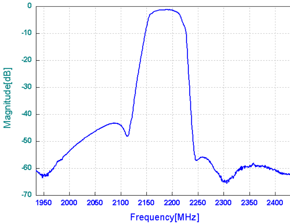
Frequency Response
